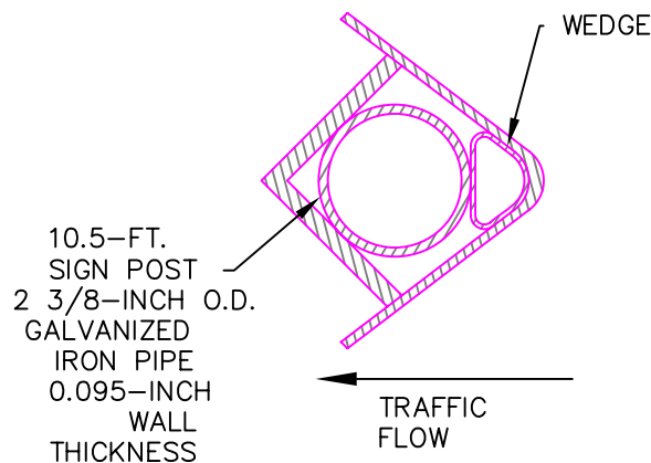
V-LOCK SIGN ANCHOR
