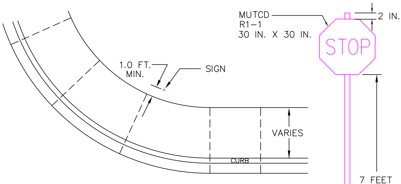
STOP SIGN PLAN VIEW
