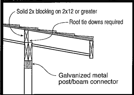
Detail C
