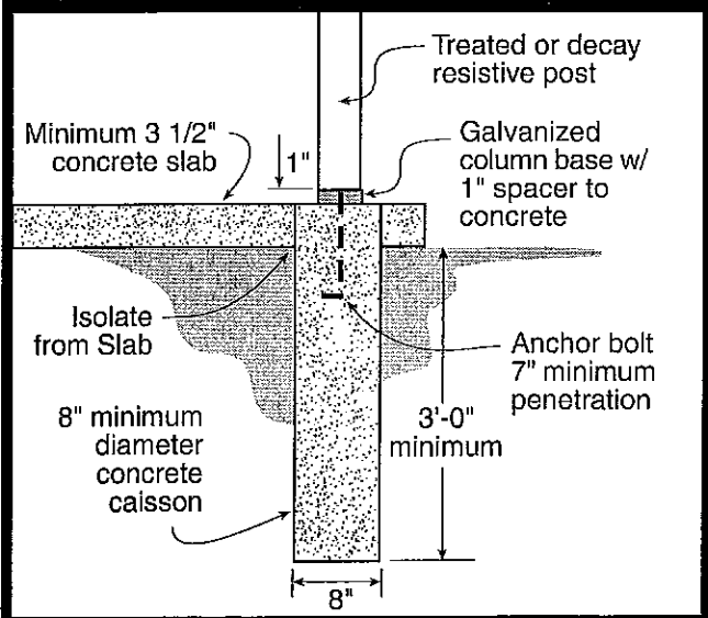
Detail C
