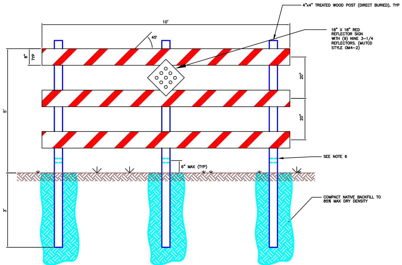
TYPE III BARRICADE DETAIL
