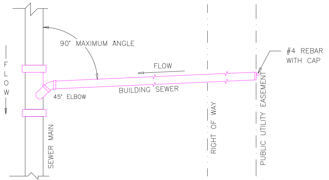
PLAN VIEW
