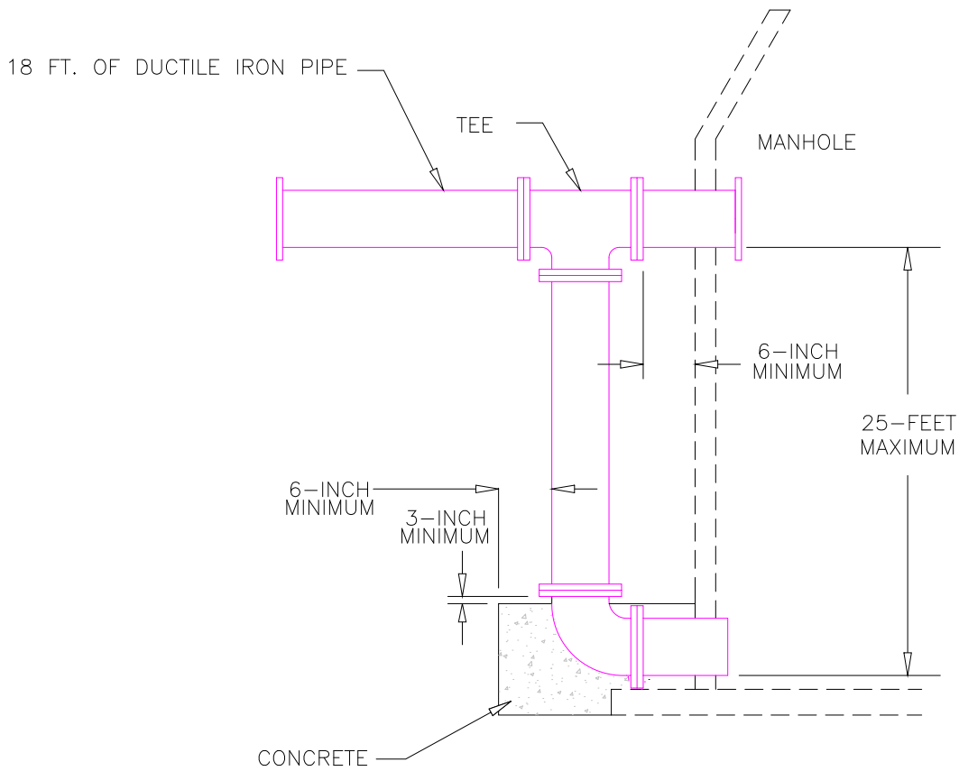
DUCTILE IRON DROP CONNECTION
